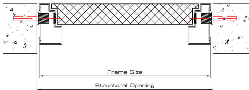
TYPICAL PLAN
