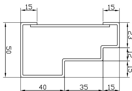
FRAME DETAIL
